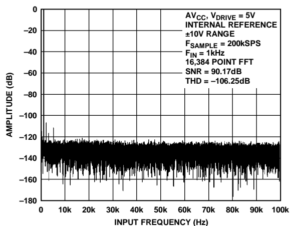
Figure 11. AD7606 FFT, ±10 V Range
