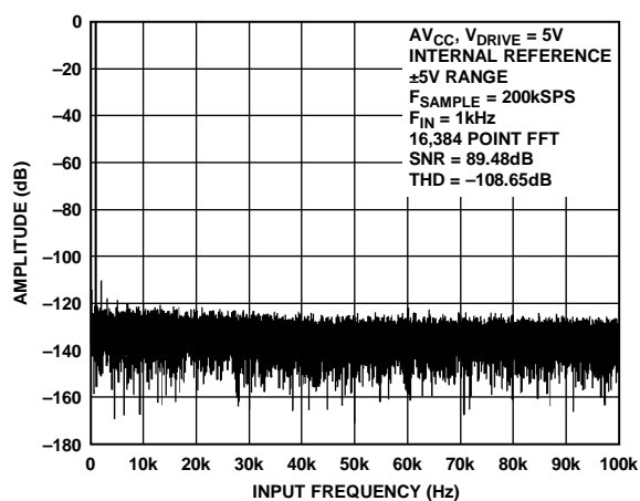
Figure 12. AD7606 FFT Plot, ±5 V Range
